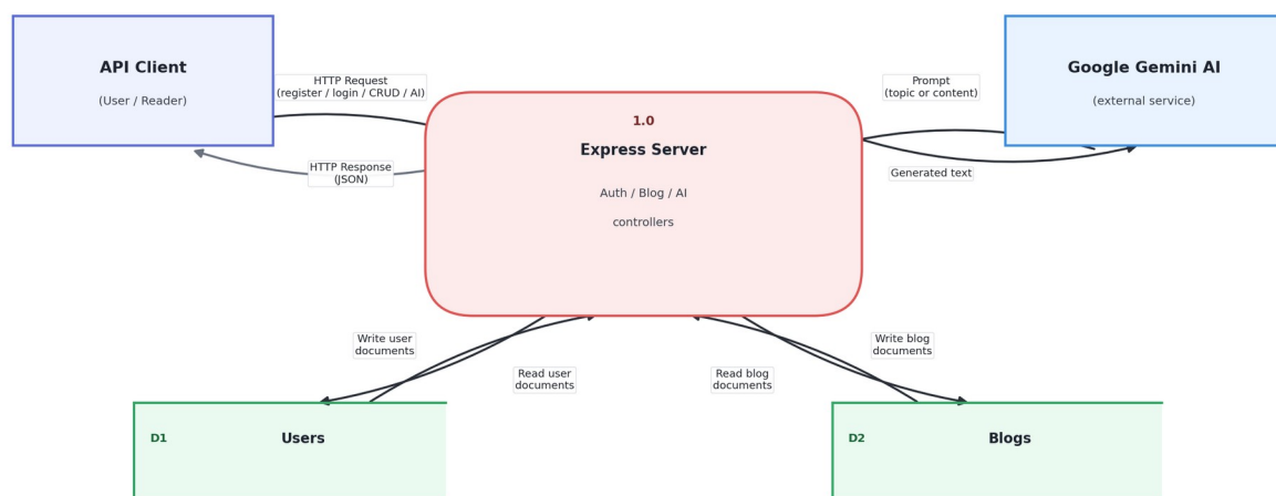
Figure 1: High-level data flow through AI BlogNest API
